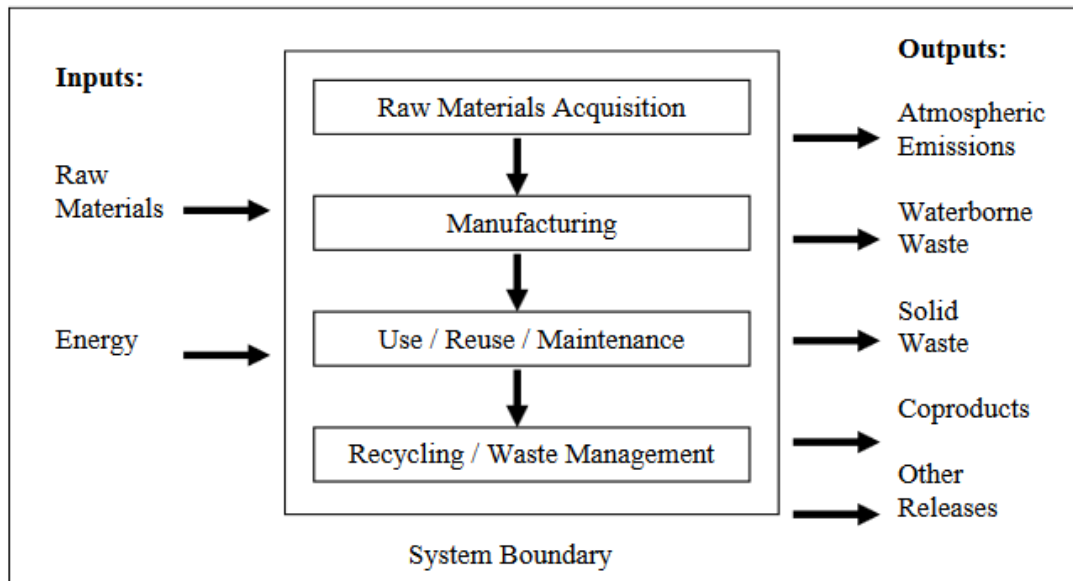
Figure 3: The Life Cycle of EPDM
